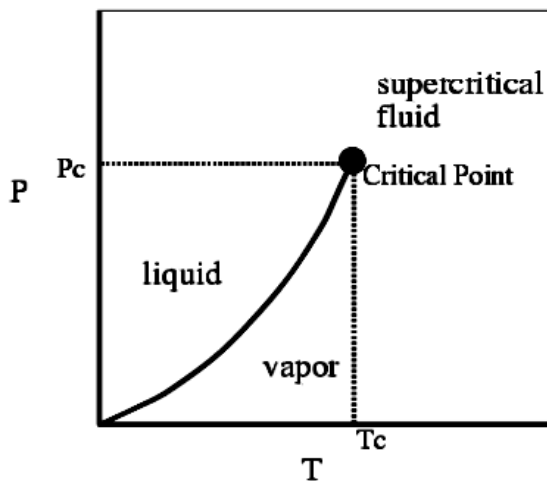
Figure 3: Critical point
