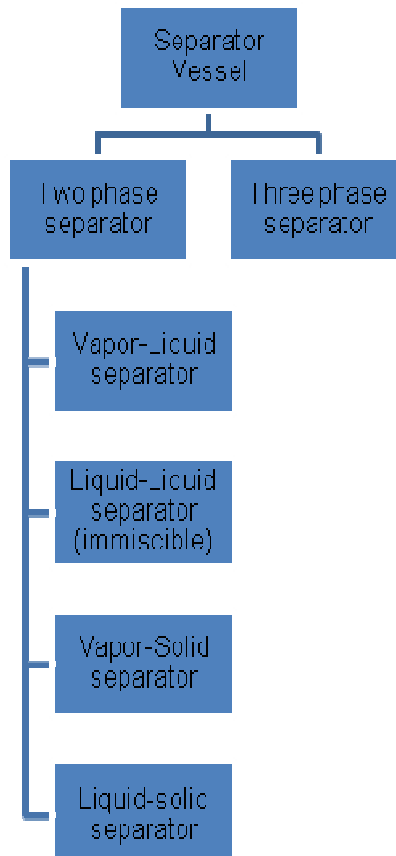
Figure 1. General types of separator vessel
