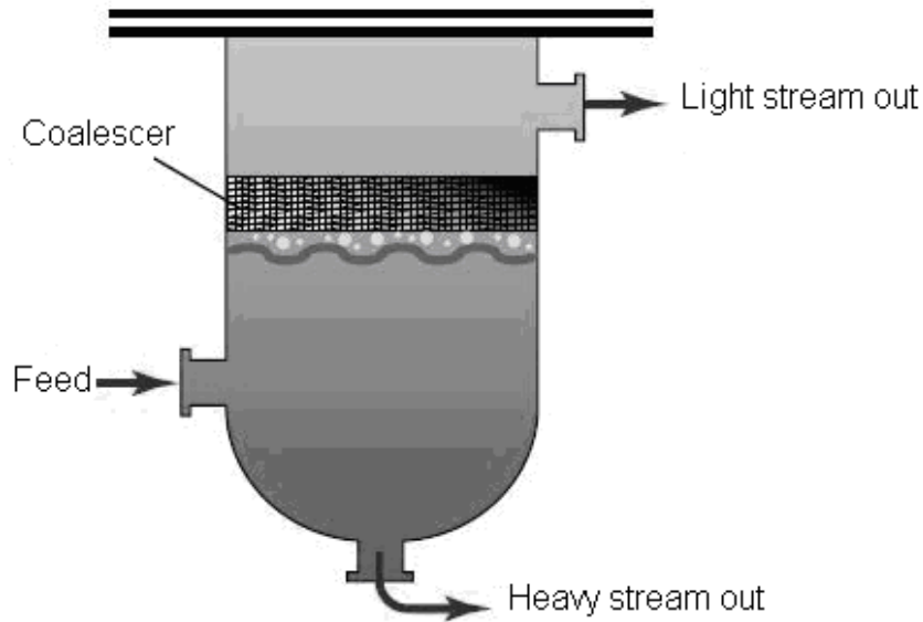
Figure 5. Vertical coalescer
