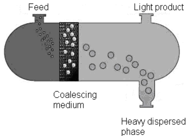
Figure 6. Horizontal coalesce
