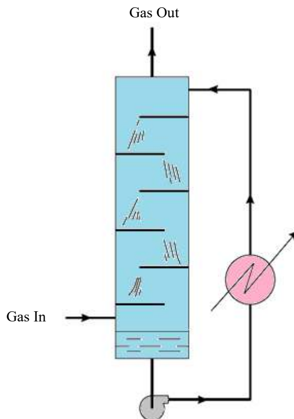
Figure 5: Typical direct-contact cooler
