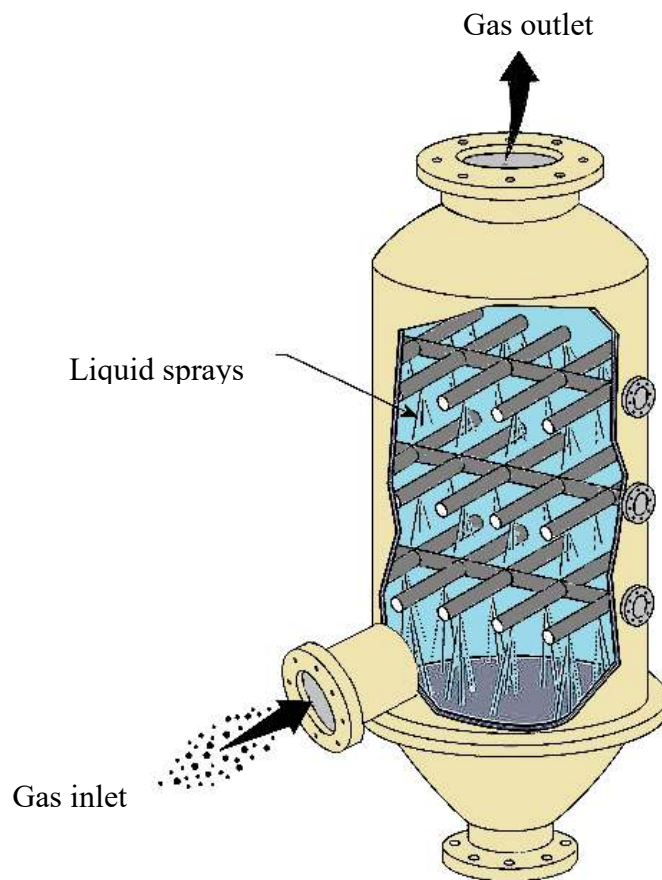
Figure 1: Spray tower
