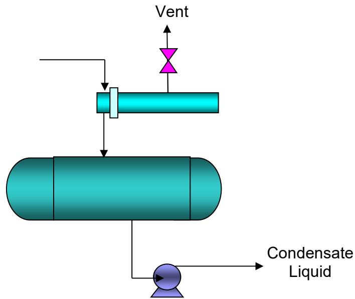
Figure 8: Total Condenser
