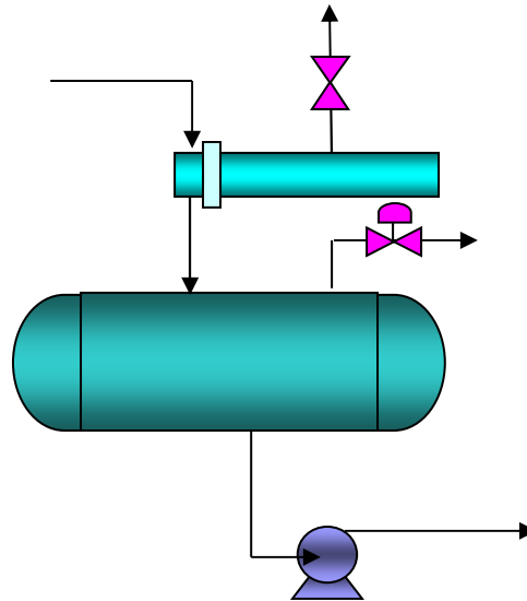
Figure 9: Partial Condenser
