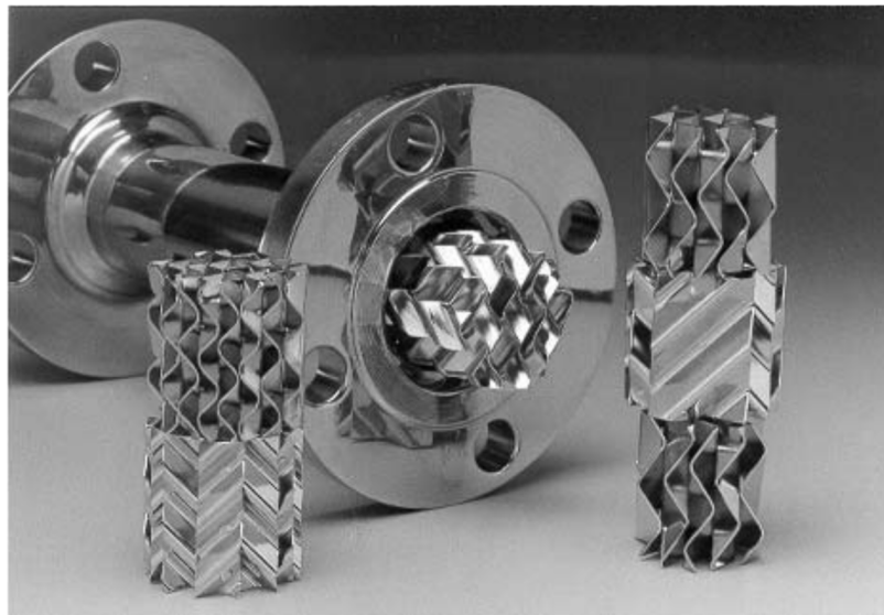
Figure 3: Corrugated plate static mixer (SMV).
