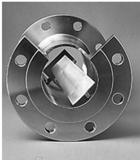
Figure 5: KVM vortex static mixer shown in flanged housing.
