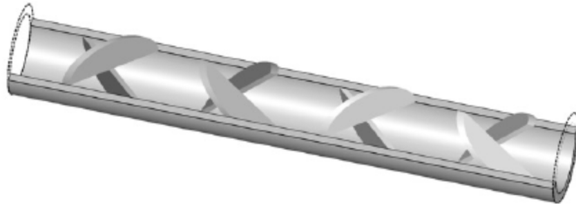
Figure 6: General R LPD (right rotation–left rotation; crossing angle \theta = 90^\circ )
